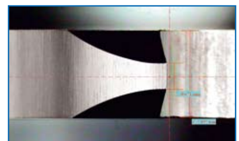
Inspection of chamfer-width / -symmetry
